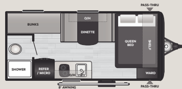
17B WEIGHT 3606 LENGTH 20' 2"
