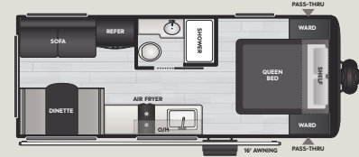
19R WEIGHT 4114 LENGTH 23' 11"
