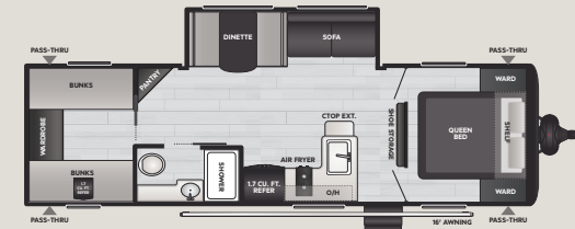
27B WEIGHT 6094 LENGTH 31' 11"
