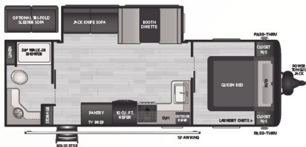
NEW! 24RBS | WEIGHT TBD | LENGTH TBD | ▪ SUPER SLIDE, REAR BATH, OUTDOOR KITCHEN
