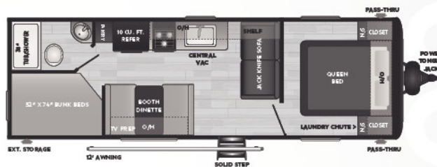
NEW! 25BHN | WEIGHT TBD | LENGTH 29' 3" | ▪ NON-SLIDE, DOUBLE BUNKS, PRIVATE BEDROOM
